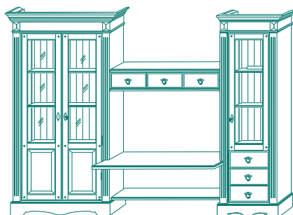
Kombination 3 278x204x57cm
